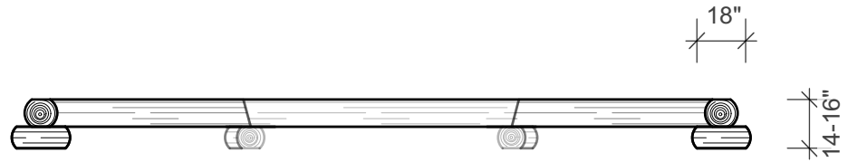
1 FRONT ELEVATION
